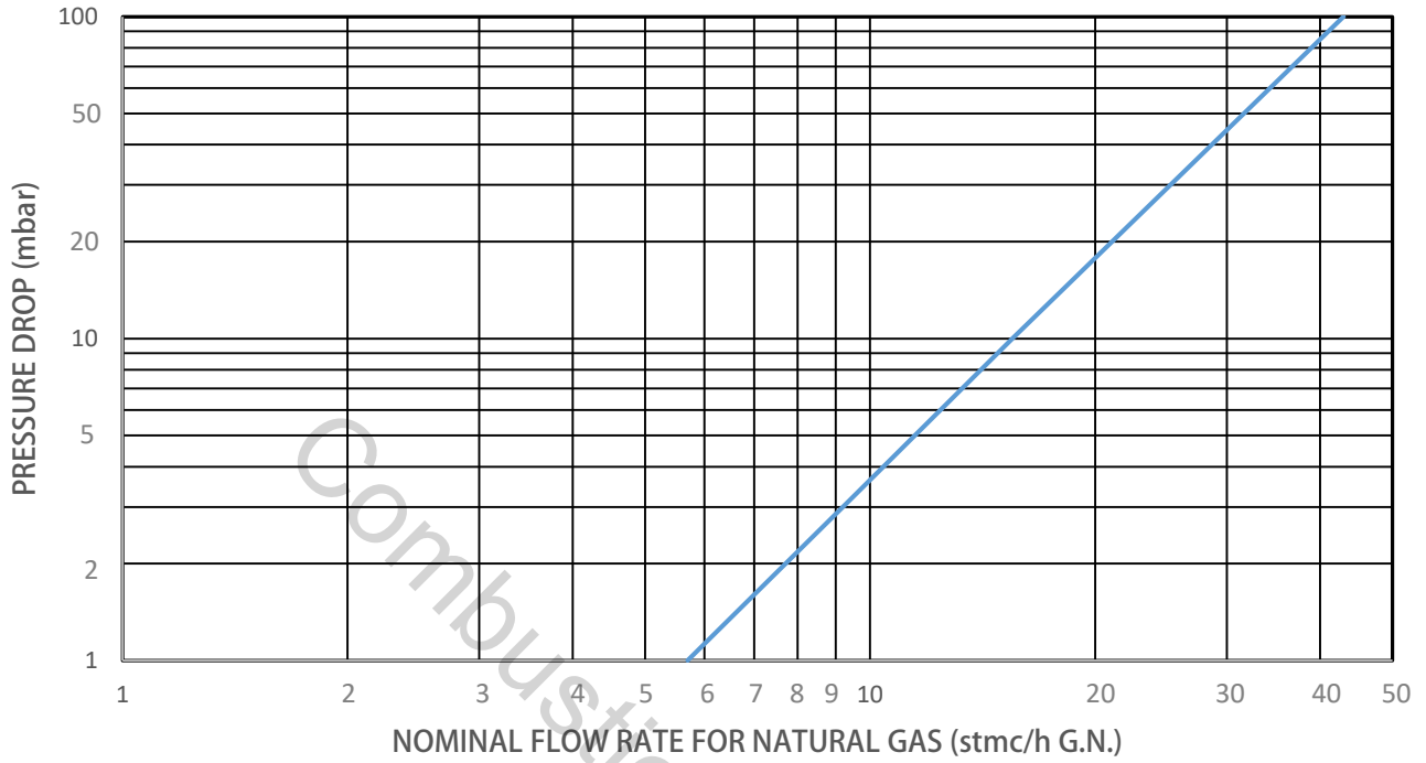
DIAGRAM FLOW RATE: 31053 - 1" FOR NATURAL GAS
