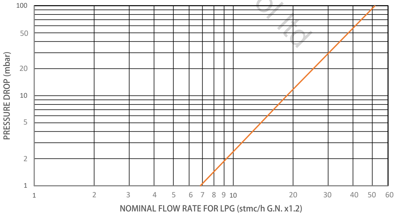
DIAGRAM FLOW RATE: 31053 - 1" FOR LPG
